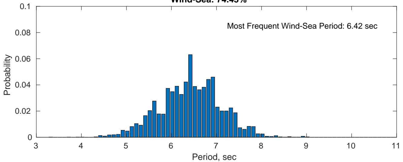
Wind-Sea: 74.43%
