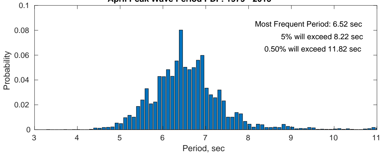
Wind-Sea: 74.43%
