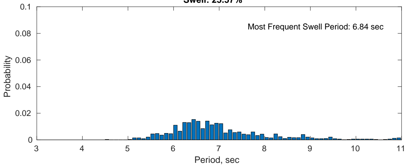
Swell: 25.57%
