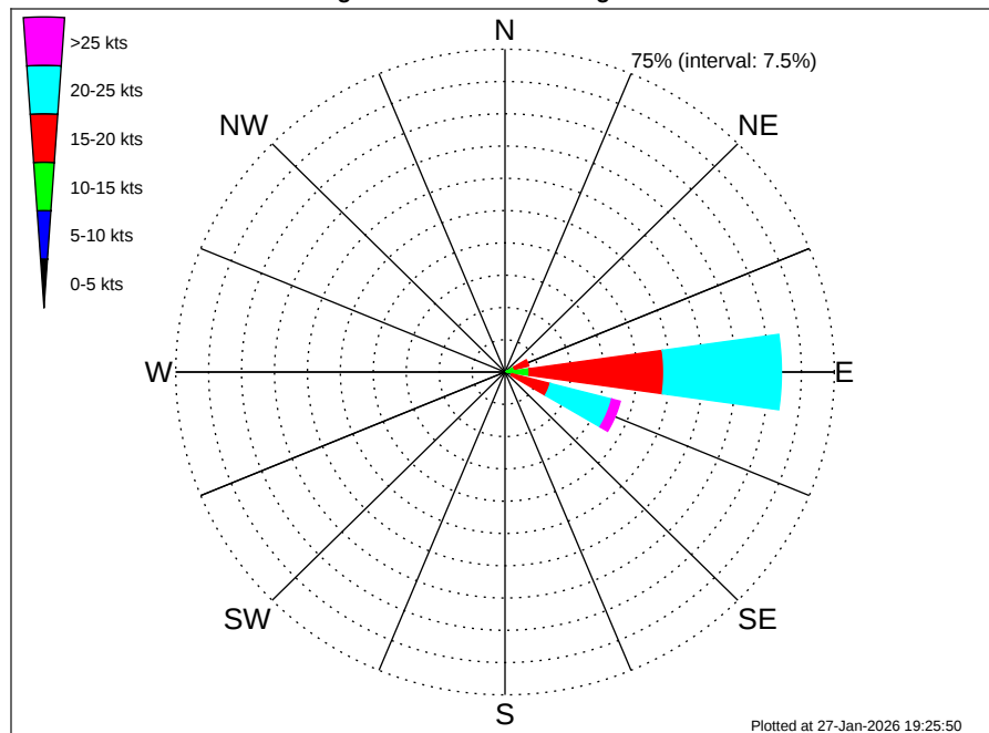
Aruba EBS Climatological Wind Rose for August: 1979 - 2015
