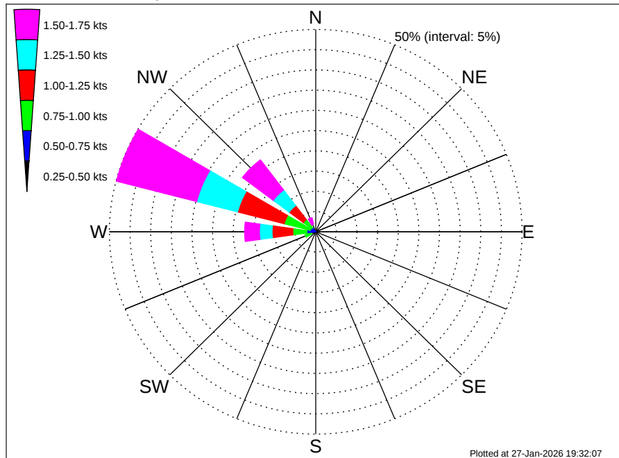
Aruba EBS Climatological Surface Current Rose for December: 1995 - 2012
