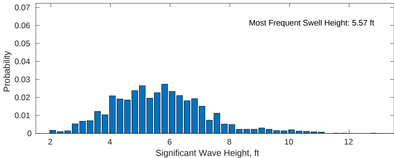
Swell: 37.17%
