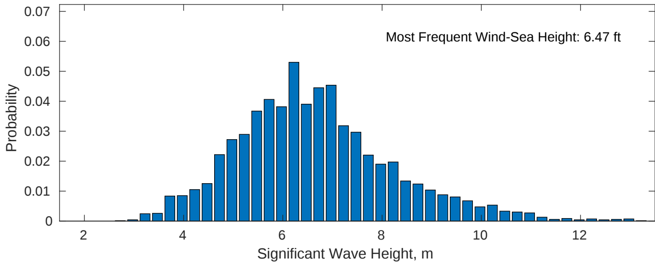
Wind-Sea: 62.83%
