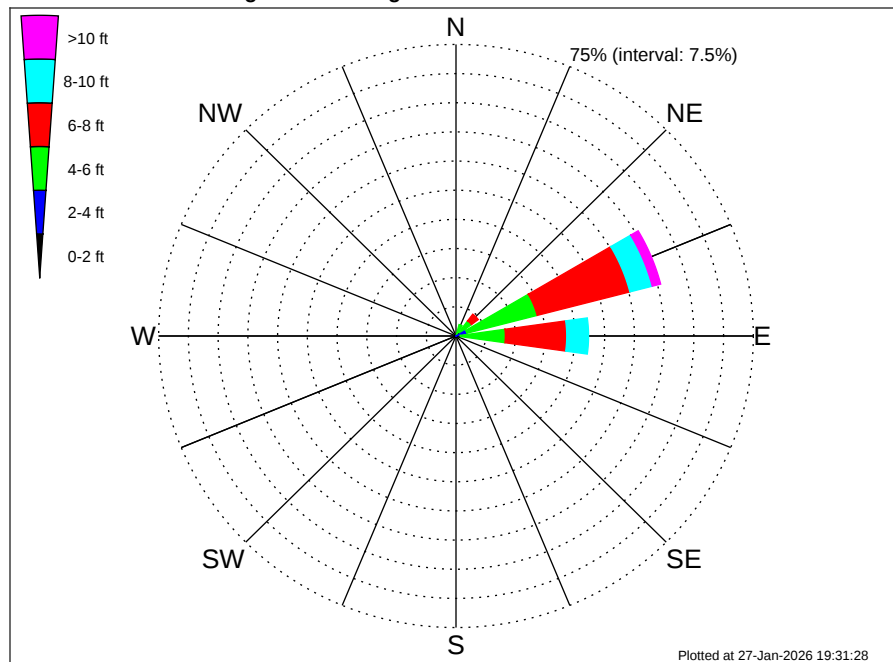
Aruba EBS Climatological WaveHeight Rose for December: 1979 - 2015
