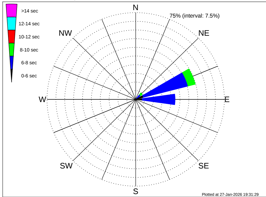
Aruba EBS Climatological WavePeriod Rose for December: 1979 - 2015
