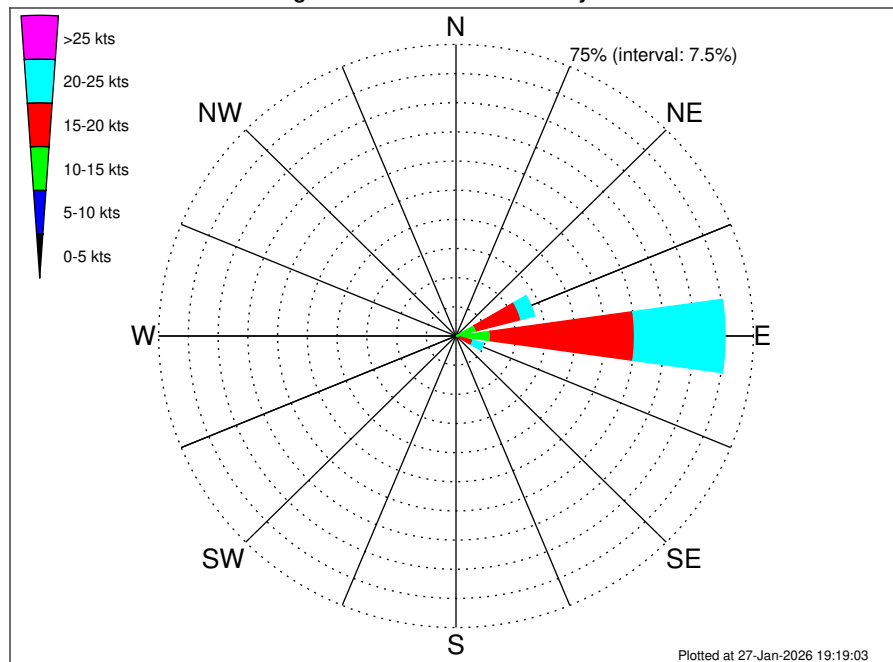
Aruba EBS Climatological Wind Rose for February: 1979 - 2015
