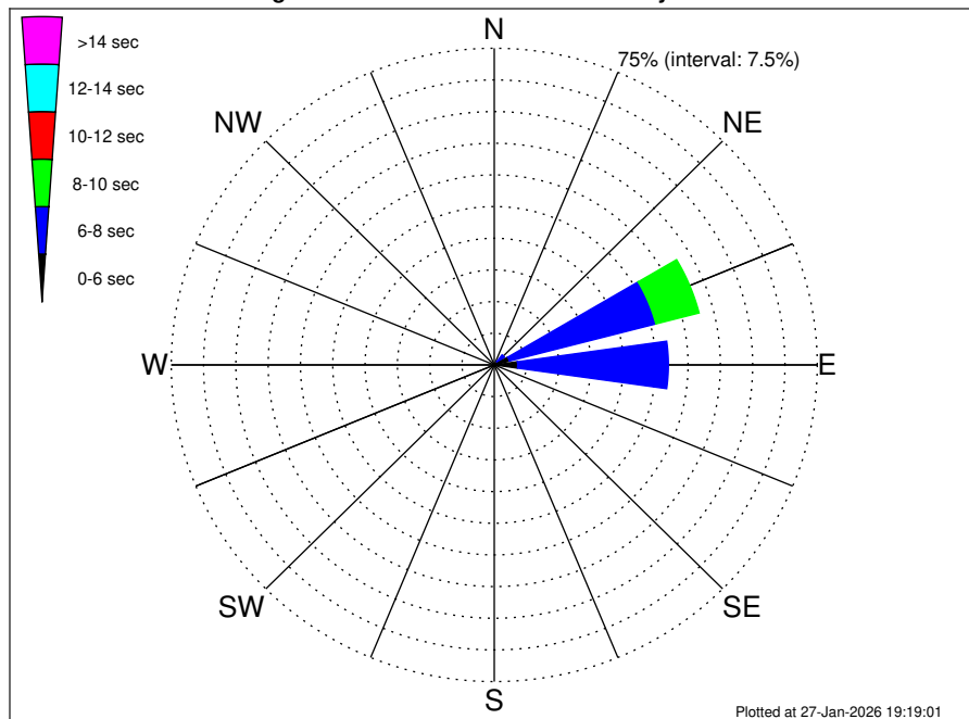
Aruba EBS Climatological WavePeriod Rose for February: 1979 - 2015
