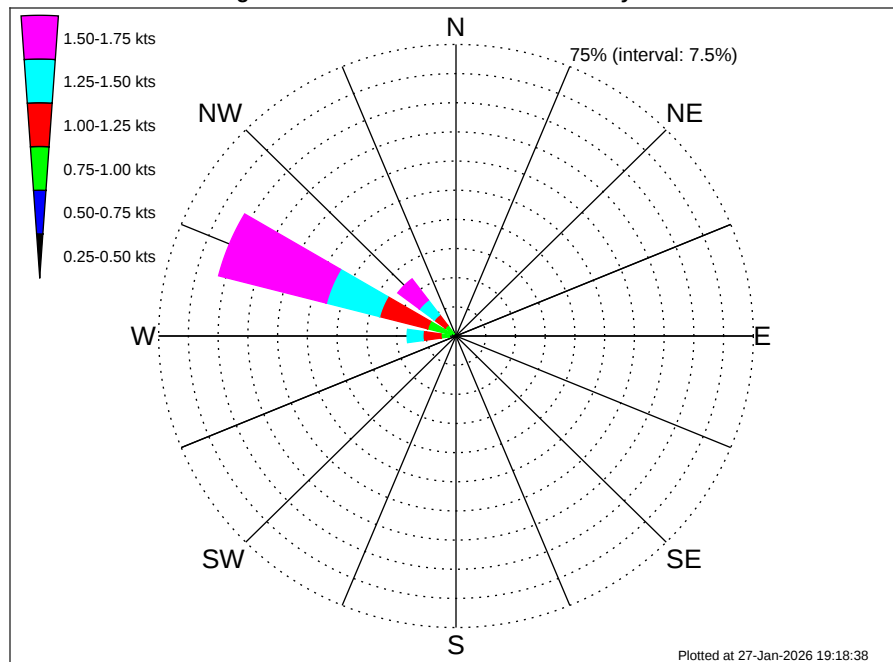
Aruba EBS Climatological Surface Current Rose for January: 1995 - 2012
