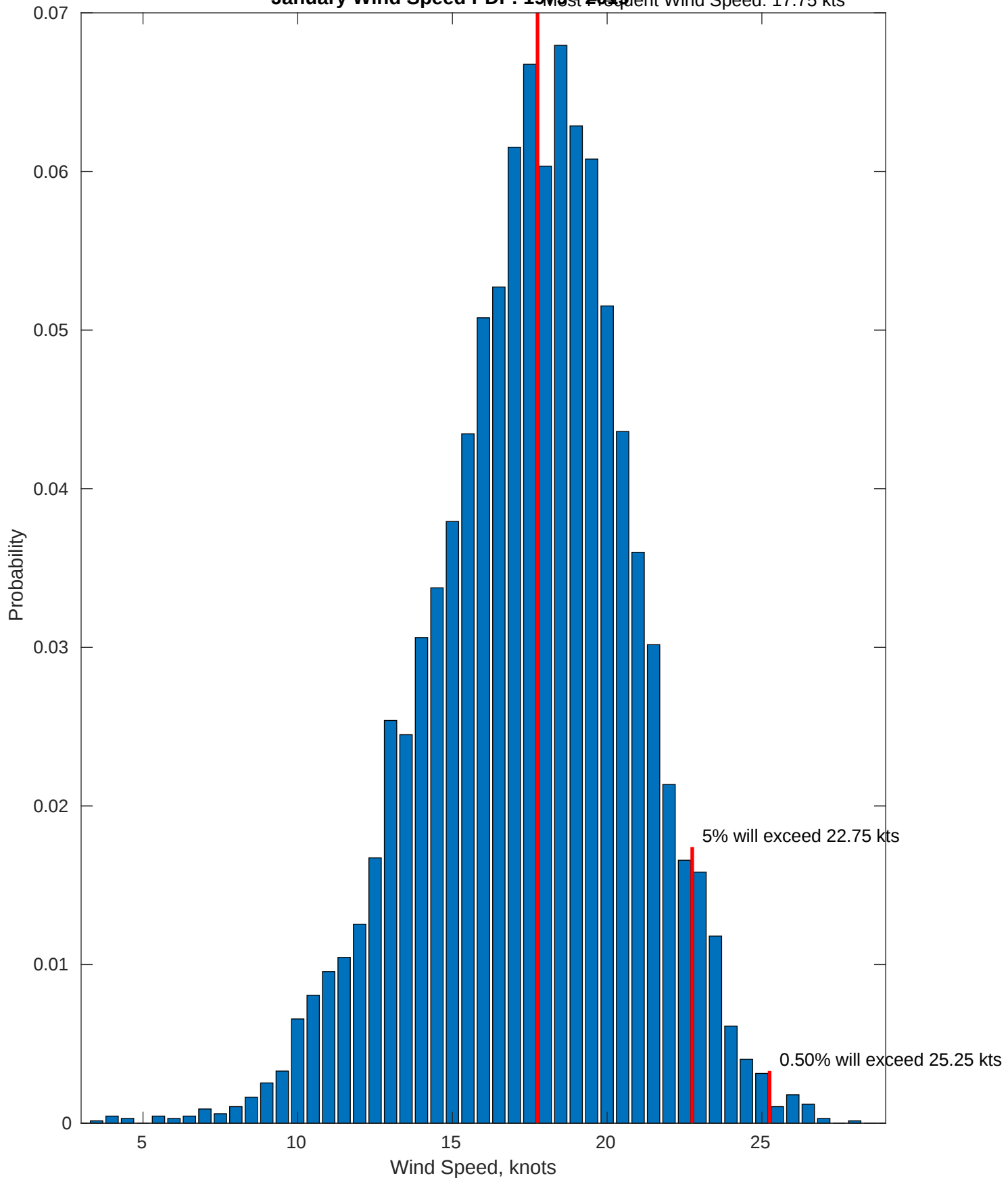
January Wind Speed PDF: 1979-2015 Most Frequent Wind Speed: 17.75 kts
