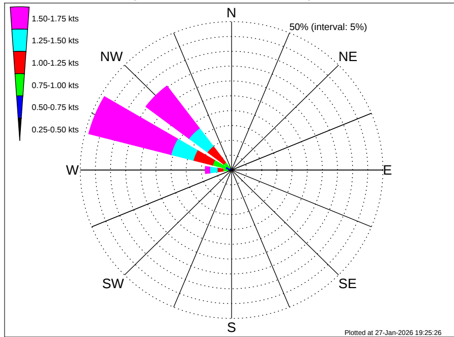
Aruba EBS Climatological Surface Current Rose for July: 1995 - 2012
