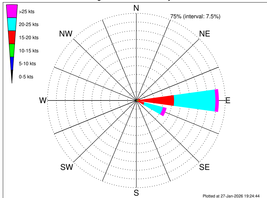
Aruba EBS Climatological Wind Rose for July: 1979 - 2015
