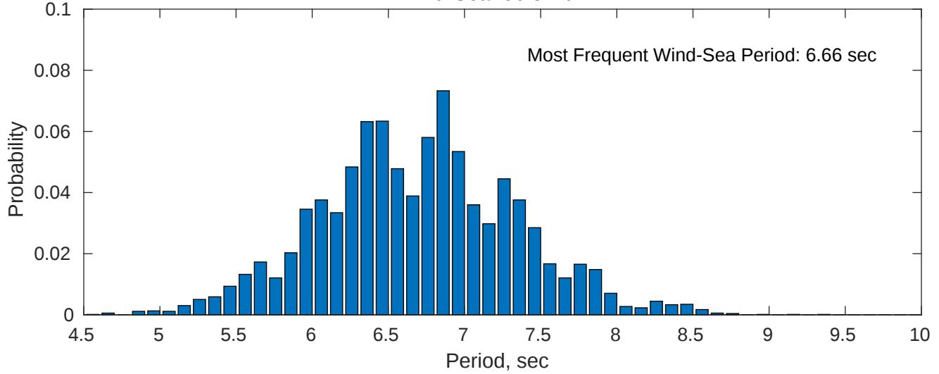
Wind-Sea: 90.57%
