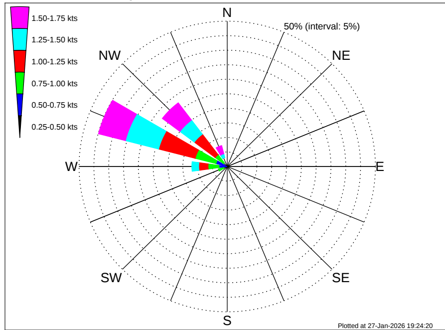
Aruba EBS Climatological Surface Current Rose for June: 1995 - 2012
