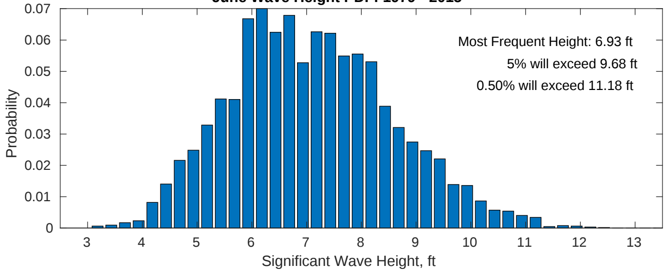
June Wave Height PDF: 1979 - 2015
