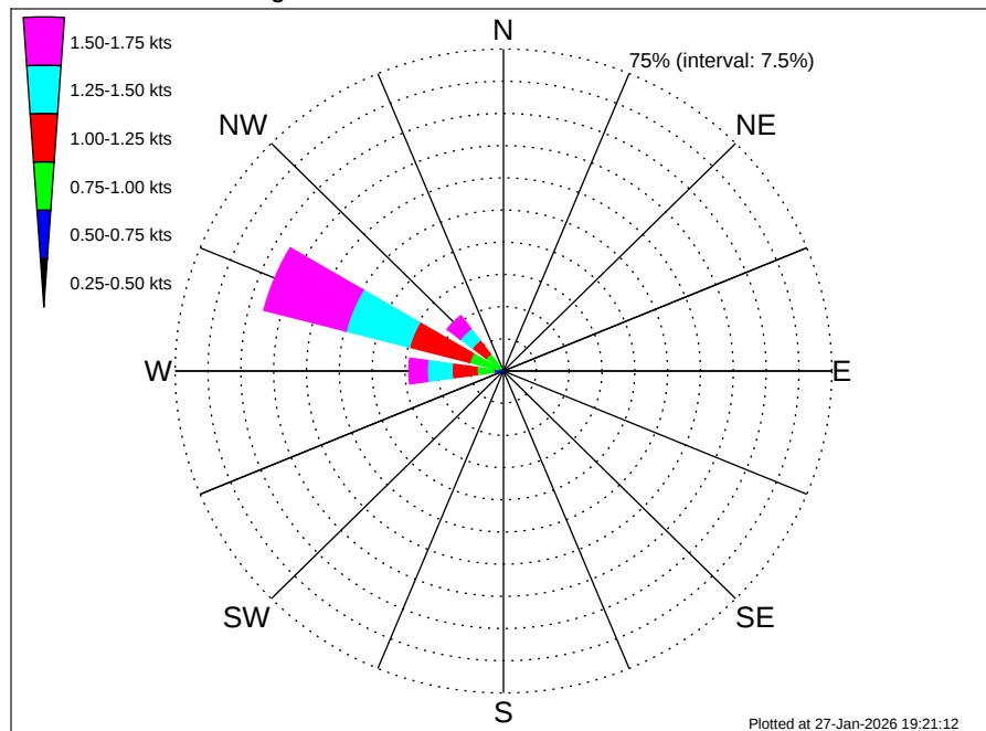
Aruba EBS Climatological Surface Current Rose for March: 1995 - 2012
