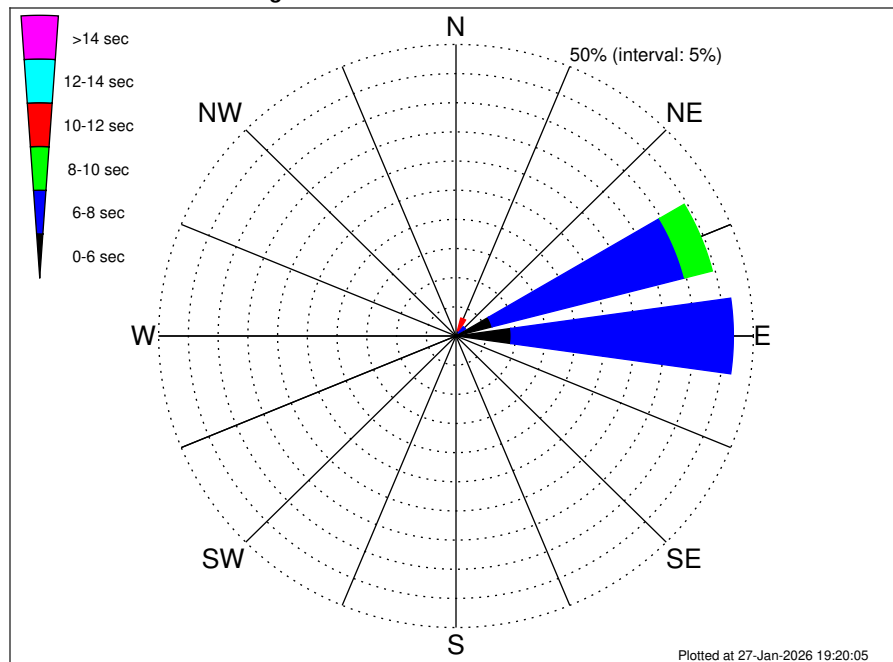
Aruba EBS Climatological WavePeriod Rose for March: 1979 - 2015
