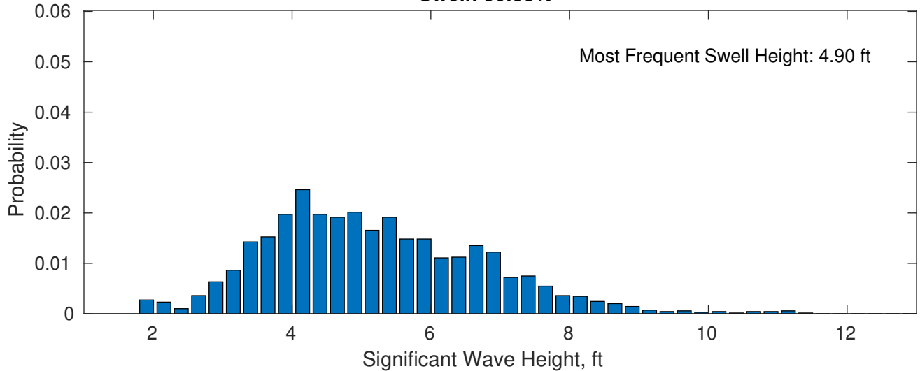
Swell: 30.83%
