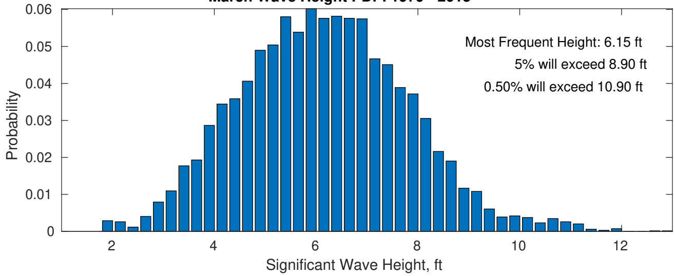
Wind-Sea: 69.17%
