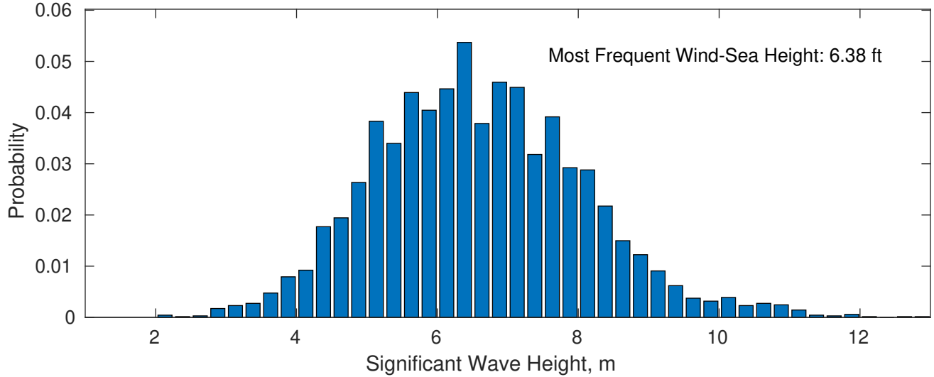
Wind-Sea: 69.17%
