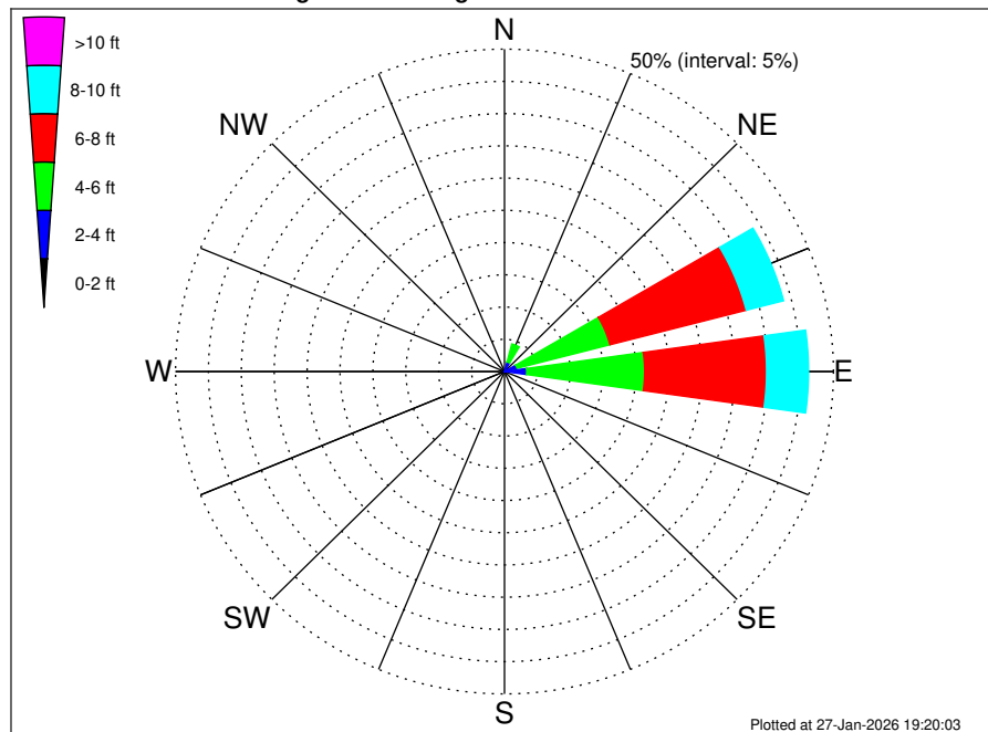
Aruba EBS Climatological WaveHeight Rose for March: 1979 - 2015
