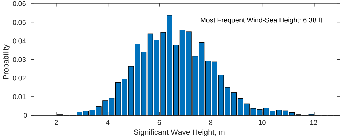
Wind-Sea: 69.17%
