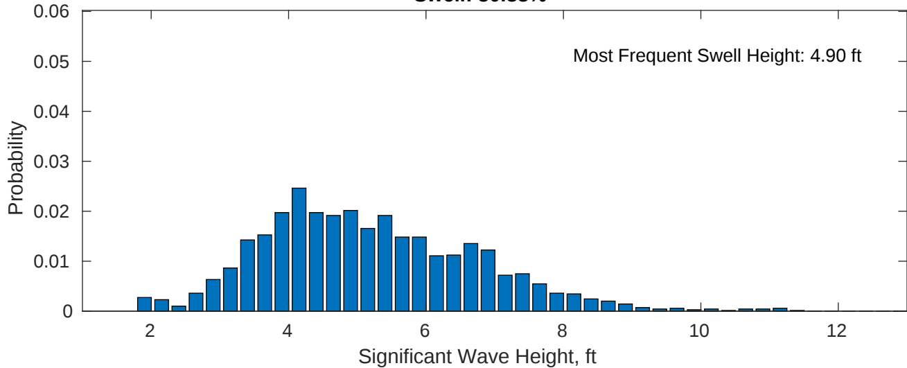
Swell: 30.83%
