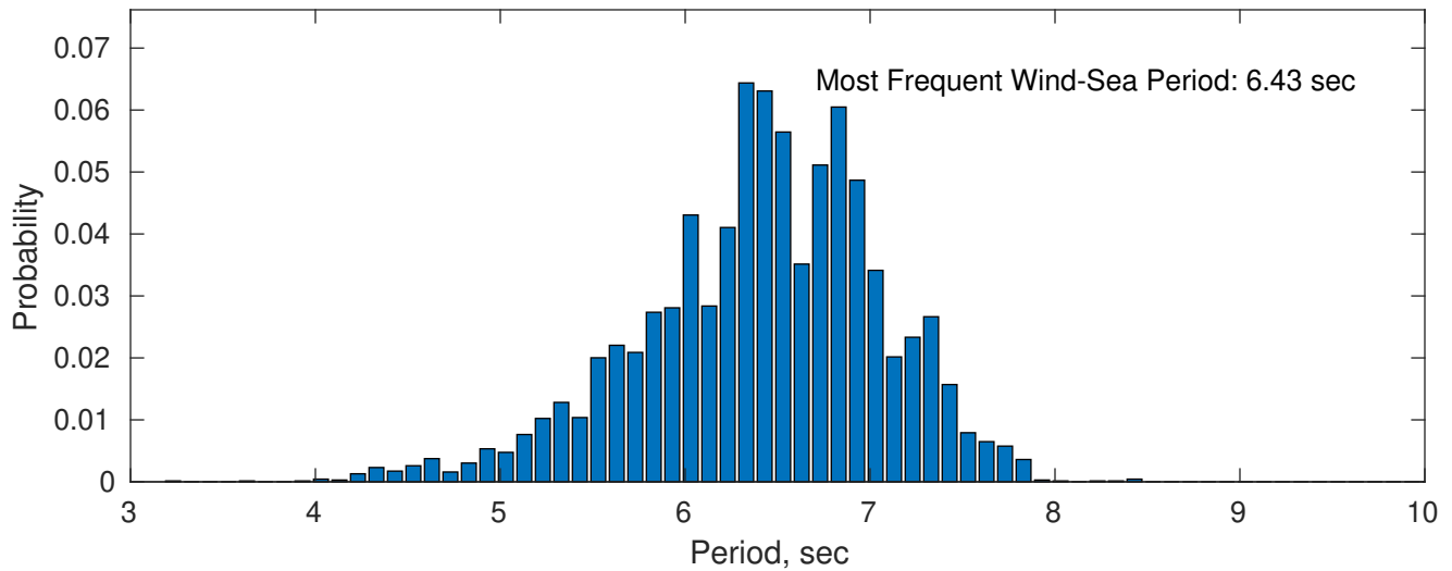
Wind-Sea: 82.36%
