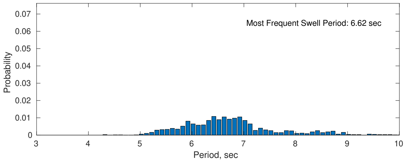
Swell: 17.64%
