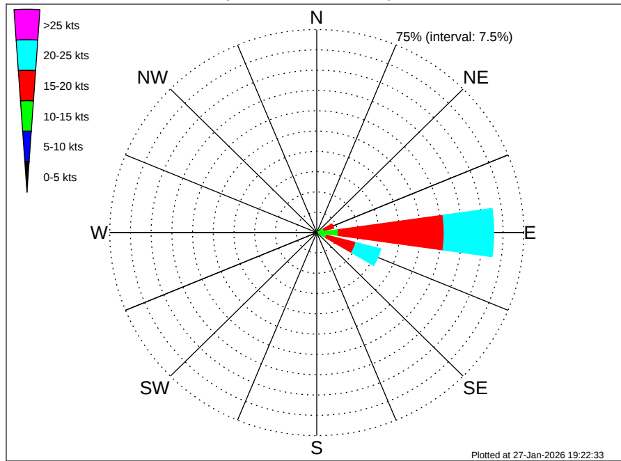
Aruba EBS Climatological Wind Rose for May: 1979 - 2015
