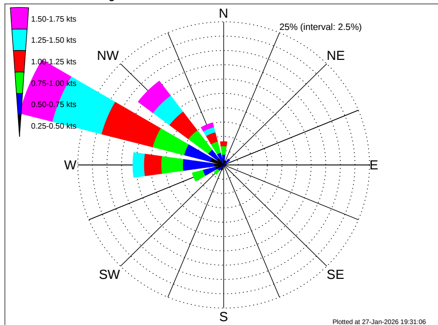
Aruba EBS Climatological Surface Current Rose for November: 1995 - 2012
