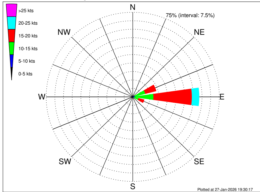
Aruba EBS Climatological Wind Rose for November: 1979 - 2015
