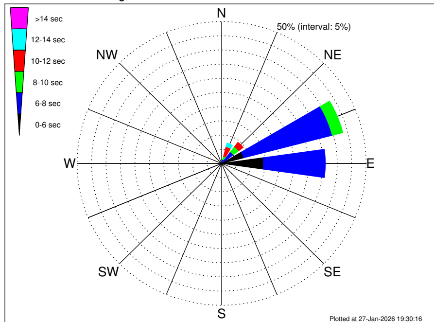
Aruba EBS Climatological WavePeriod Rose for November: 1979 - 2015
