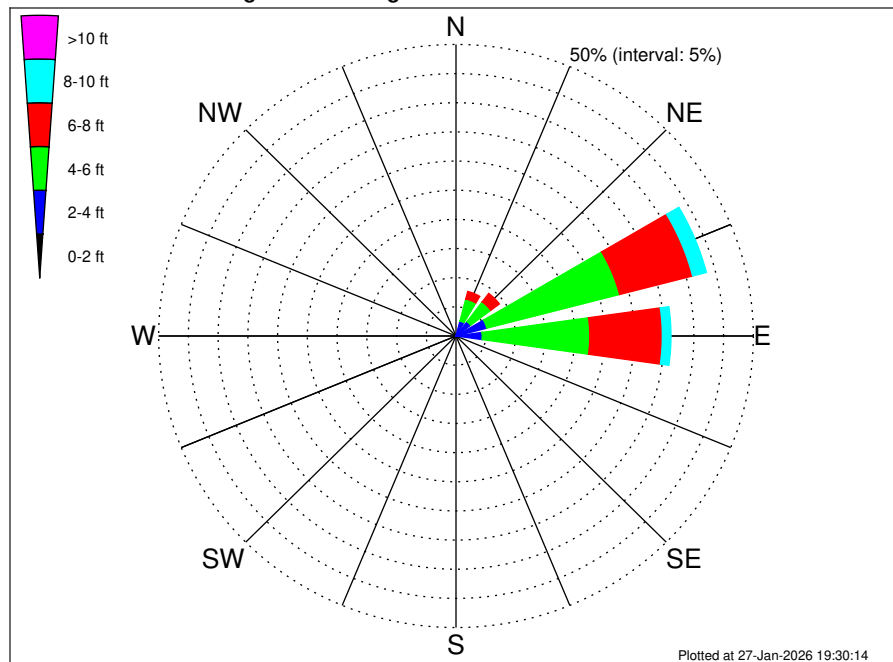
Aruba EBS Climatological WaveHeight Rose for November: 1979 - 2015
