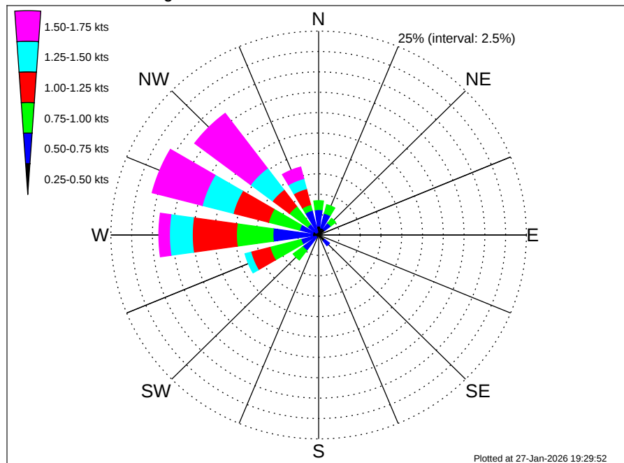
Aruba EBS Climatological Surface Current Rose for October: 1995 - 2012
