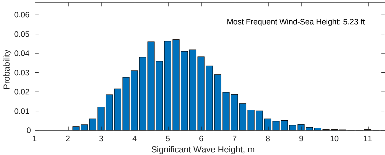
Wind-Sea: 61.74%
