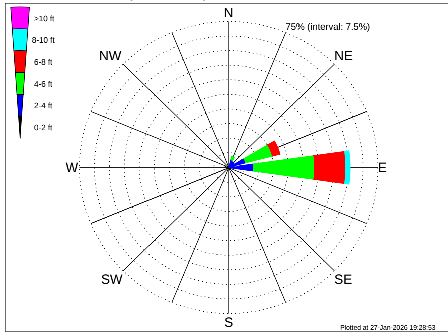
Aruba EBS Climatological WaveHeight Rose for October: 1979 - 2015
