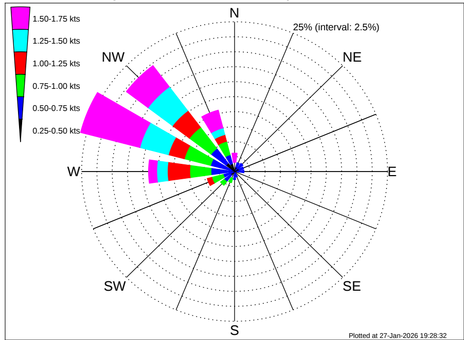
Aruba EBS Climatological Surface Current Rose for September: 1995 - 2012
