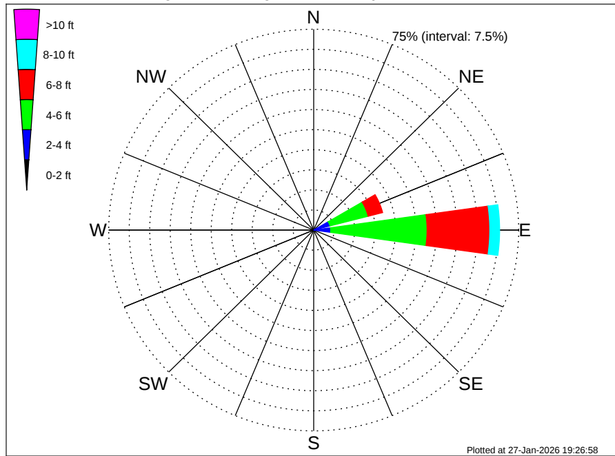
Aruba EBS Climatological WaveHeight Rose for September: 1979 - 2015
