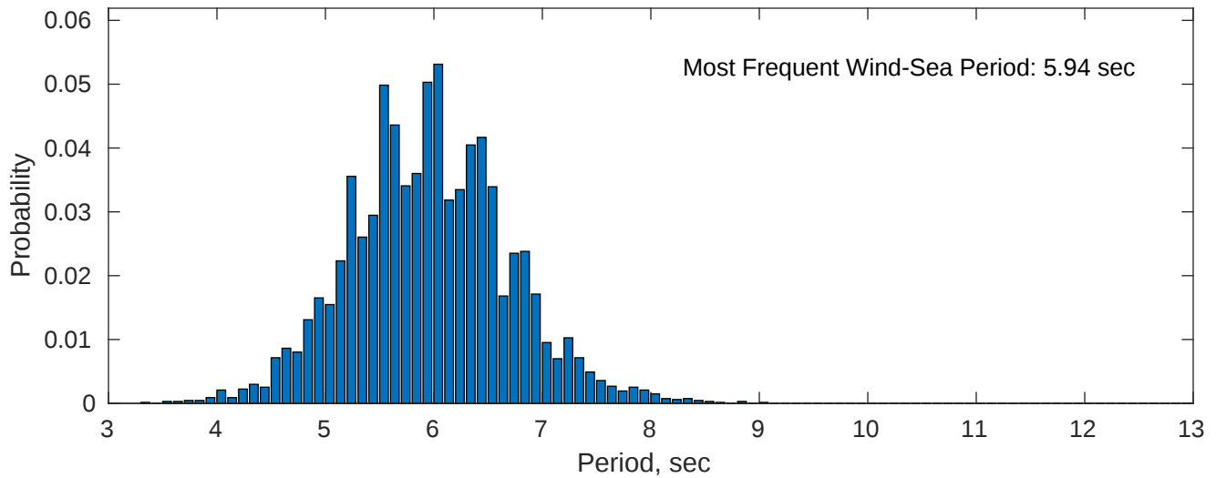
Wind-Sea: 78.17%
