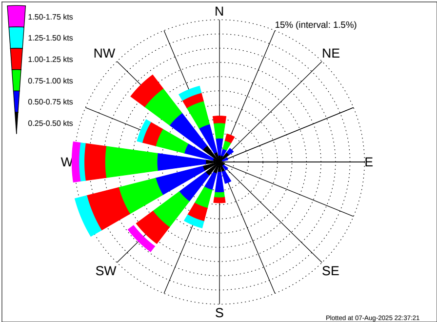
Cape Verde Islands MBES Climatological Surface Current Rose for December: 1995 - 2012
