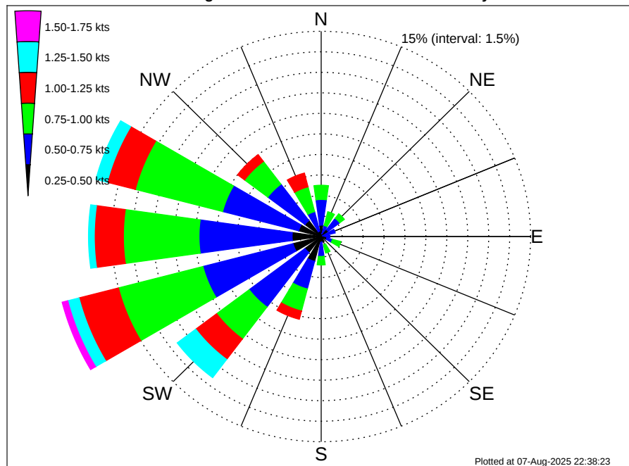
Cape Verde Islands MBES Climatological Surface Current Rose for February: 1995 - 2012
