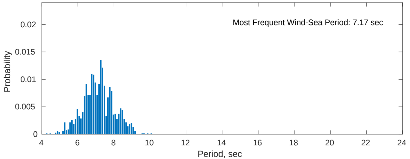
Wind-Sea: 20.41%
