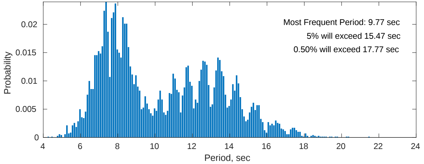
February Peak Wave Period PDF: 1979 - 2015
