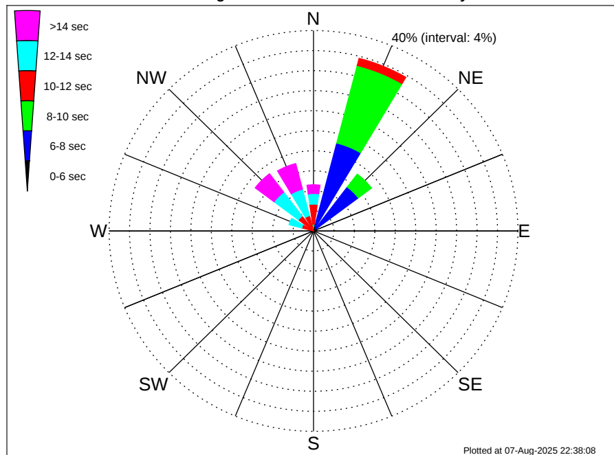
Cape Verde Islands MBES Climatological WavePeriod Rose for February: 1979 - 2015
