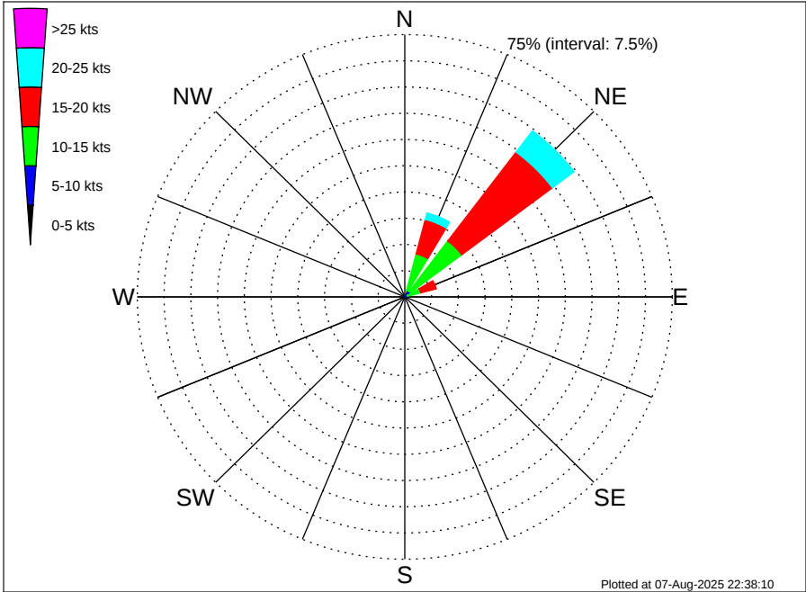
Cape Verde Islands MBES Climatological Wind Rose for February: 1979 - 2015
