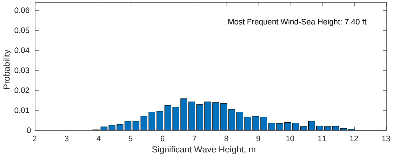
Wind-Sea: 21.98%
