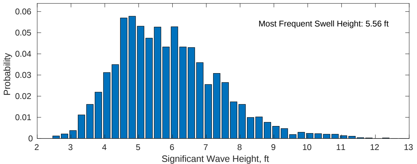
Swell: 78.02%
