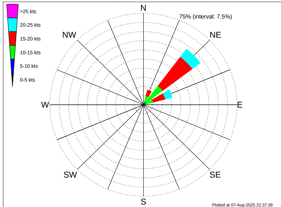
Cape Verde Islands MBES Climatological Wind Rose for January: 1979 - 2015
