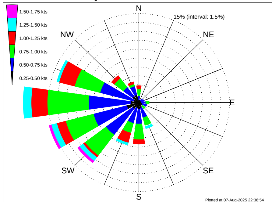
Cape Verde Islands MBES Climatological Surface Current Rose for March: 1995 - 2012
