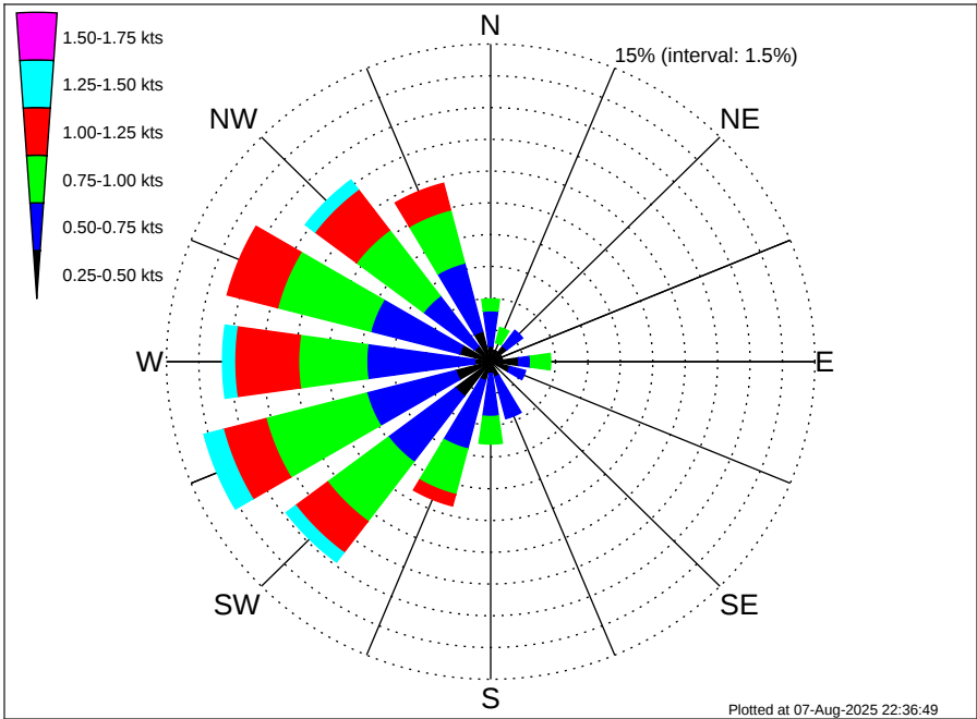
Cape Verde Islands MBES Climatological Surface Current Rose for November: 1995 - 2012
