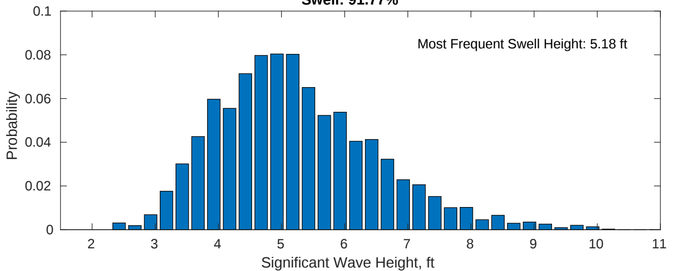
Swell: 91.77%
