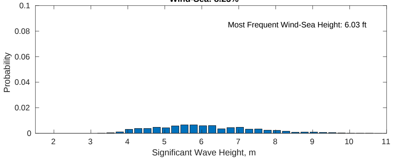
Wind-Sea: 8.23%
