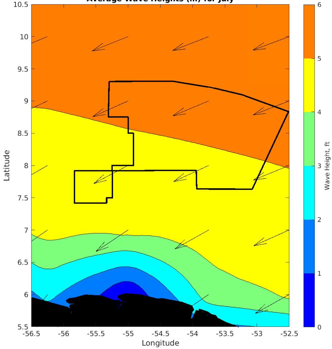
Average Wave Heights (m) for July
