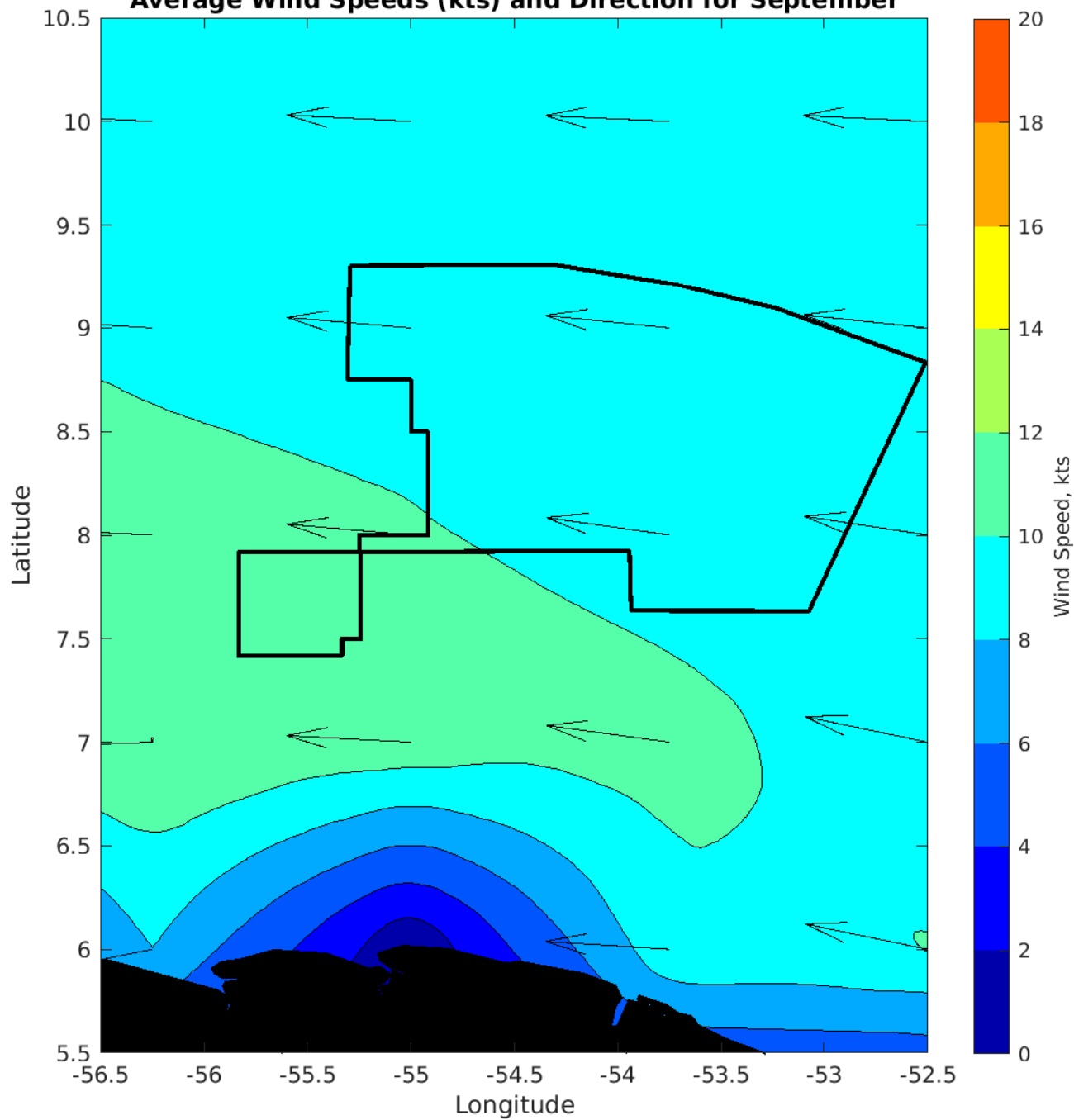
Average Wind Speeds (kts) and Direction for September
