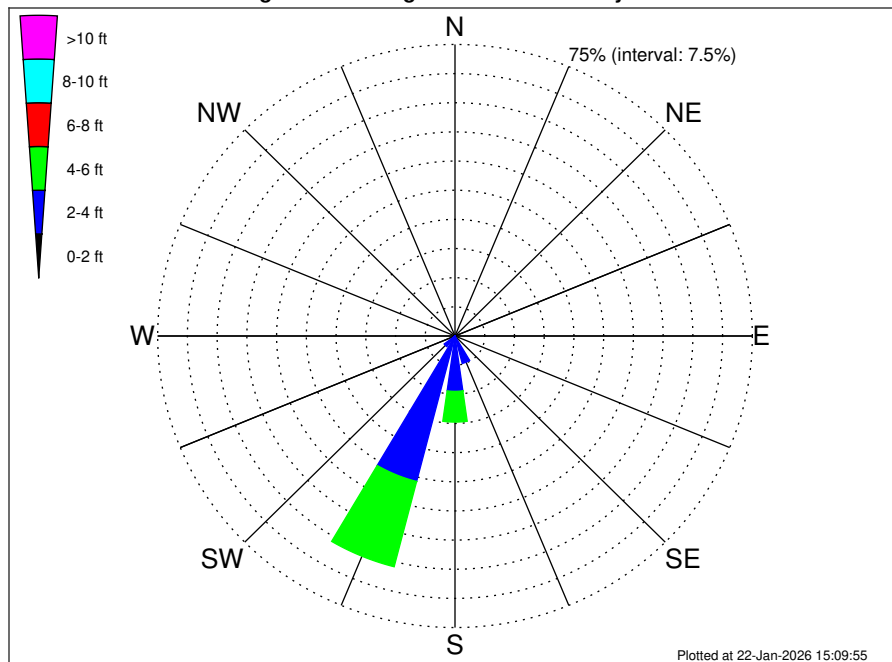
Liberia MBES Climatological WaveHeight Rose for February: 1979 - 2015
