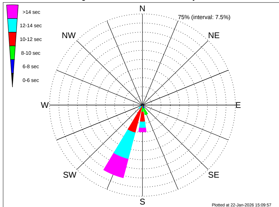
Liberia MBES Climatological WavePeriod Rose for February: 1979 - 2015
