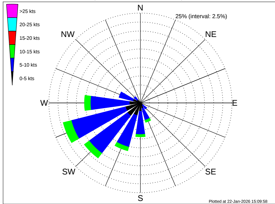
Liberia MBES Climatological Wind Rose for February: 1979 - 2015
