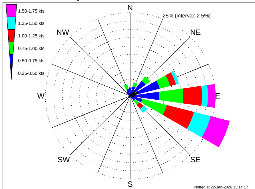
Liberia MBES Climatological Surface Current Rose for June: 1995 - 2012
