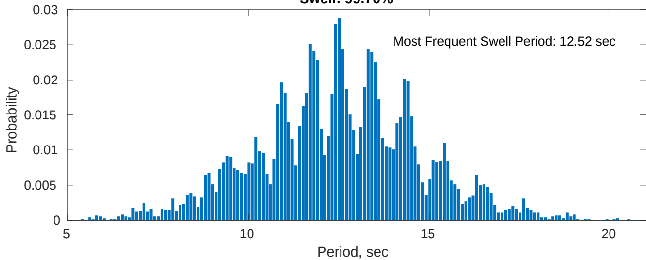
Swell: 99.70%
