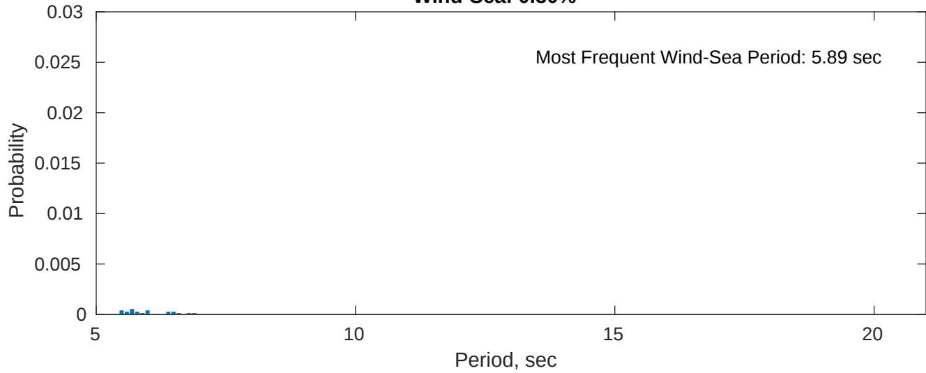
Wind-Sea: 0.30%
