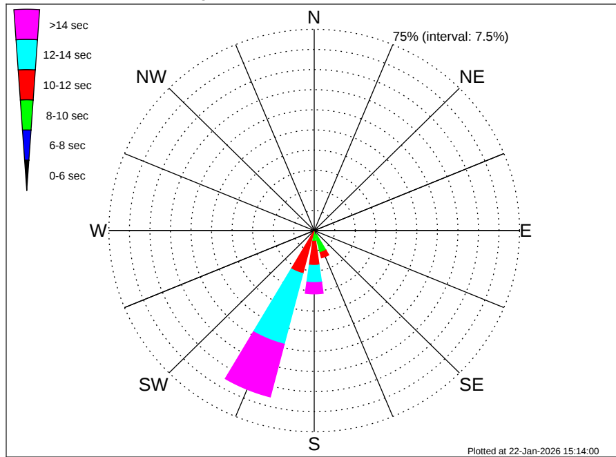
Liberia MBES Climatological WavePeriod Rose for June: 1979 - 2015
