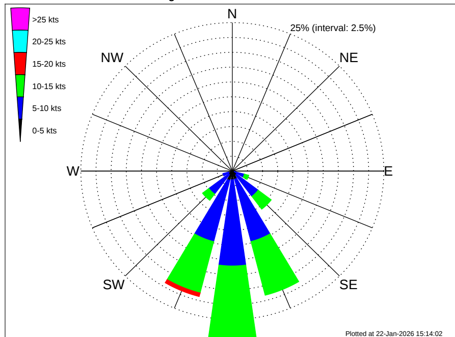
Liberia MBES Climatological Wind Rose for June: 1979 - 2015
