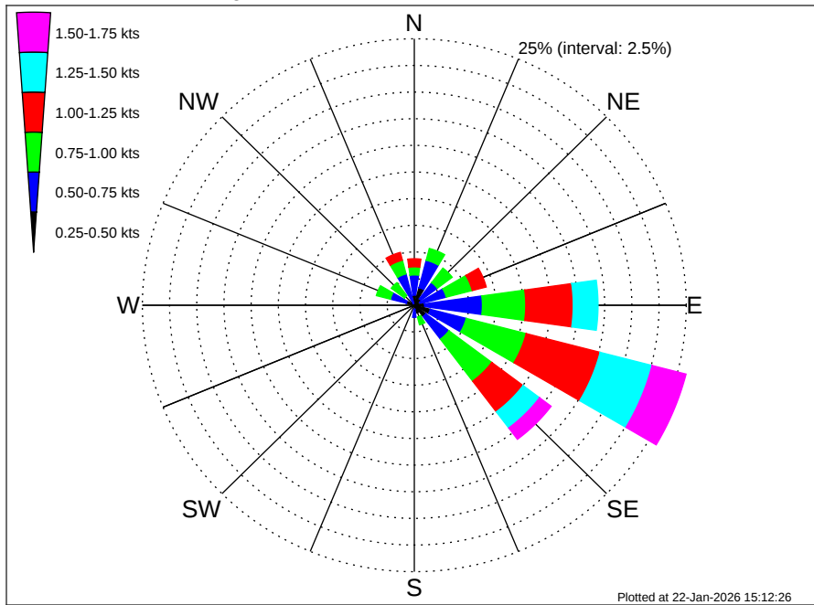
Liberia MBES Climatological Surface Current Rose for March: 1995 - 2012
