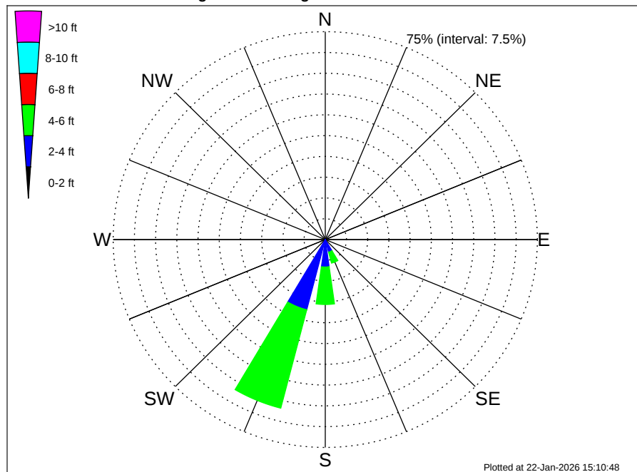
Liberia MBES Climatological WaveHeight Rose for March: 1979 - 2015
