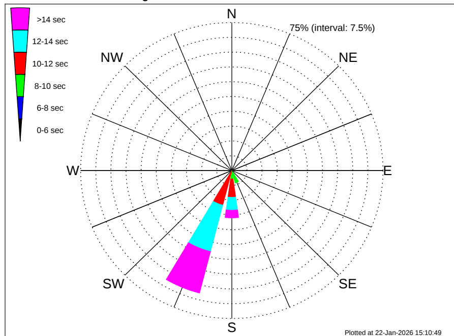
Liberia MBES Climatological WavePeriod Rose for March: 1979 - 2015
