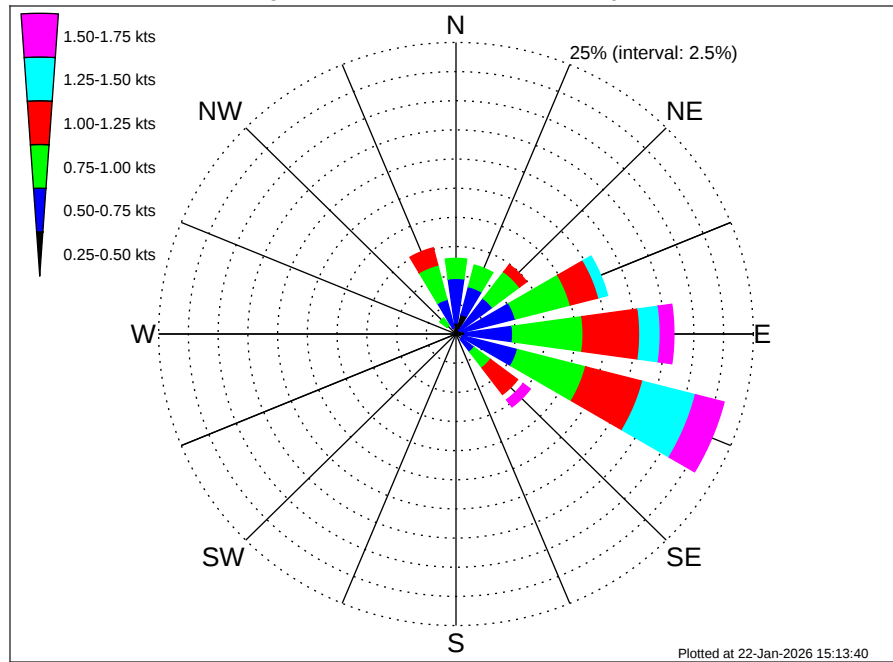
Liberia MBES Climatological Surface Current Rose for May: 1995 - 2012
